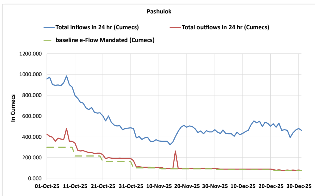
Figure 8: Graphs showing status of implementation of E-Flow at Pashulok Barrage
