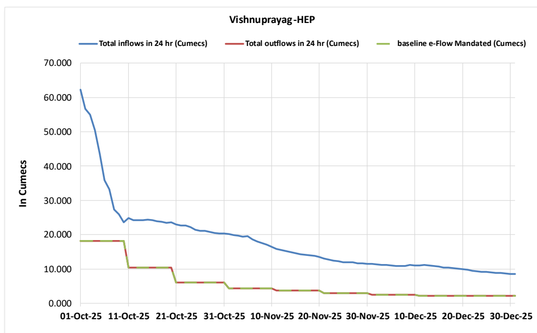
Figure 5: Graphs showing status of implementation of E-Flow at Vishnuprayag HEP
