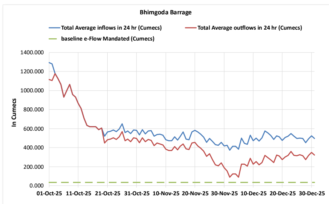
Figure 9: Graph showing status of implementation of E-Flow at Bhimgoda Barrage
