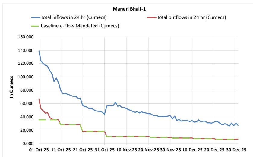
Figure 2: Graphs showing status of implementation of E-Flow at Maneri Bhal- I
