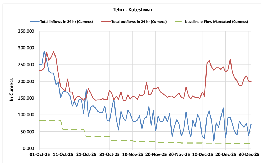
Figure 4: Graphs showing status of implementation of E-Flow at Tehri – Koteswar
