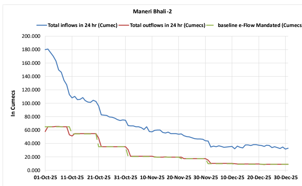
Figure 3: Graphs showing status of implementation of E-Flow at Maneri Bhal- II
